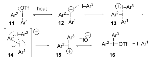
Scheme 2. Mechanistic hypothesis for the iodonium metathesis reaction.
