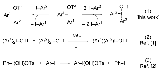
Scheme 1. Iodonium metathesis reactions.
